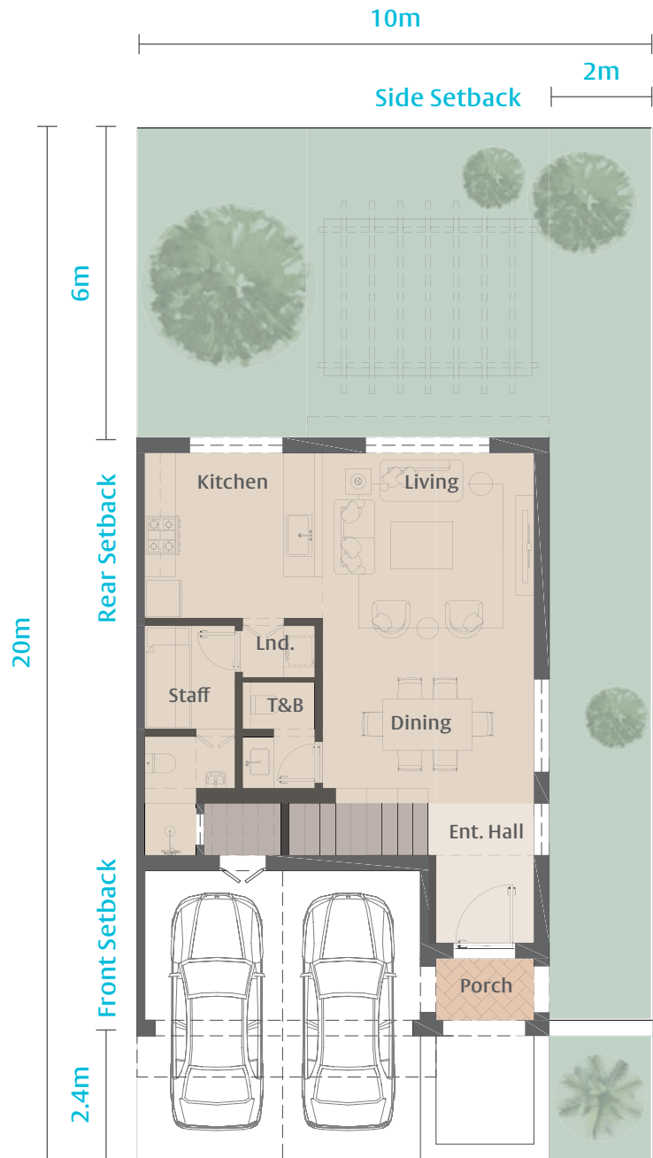
Ground Floor
